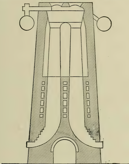
From "The American Petroleum Industry," by Bacon and Hamor. FIG. 83.—Young & Beilby Retort for Distilling Shales.
